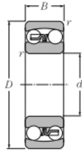
Cylindrical bore
